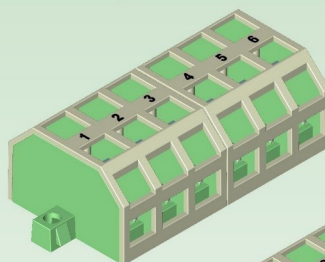
FASTON 18 POLI
